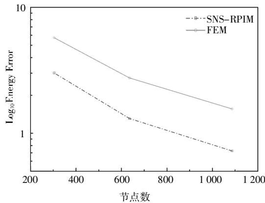
图 8 稳定 Node-based 光滑径向基点插值法与有限元法在不同节点数下的能量误差 Fig.8 Energy error of SNS-RPIM and FEM with different number of nodes
